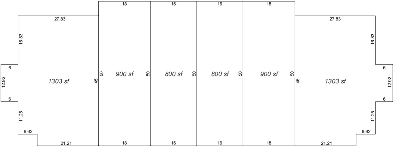
BUILDING FOOTPRINT C
