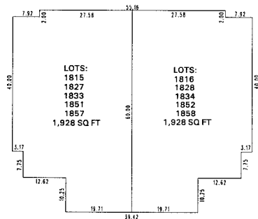
LOT DETAIL "C"
