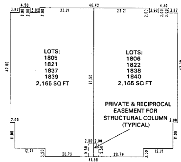
LOT DETAIL "D"
