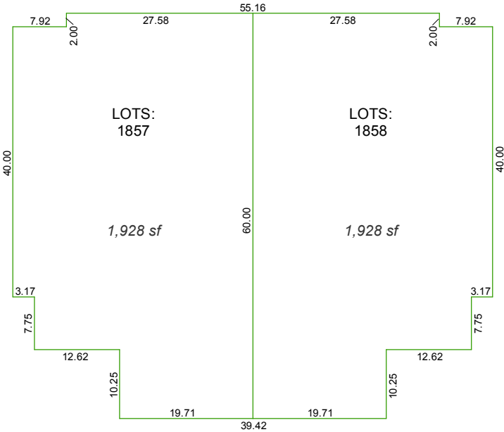
LOT DETAIL "C"
