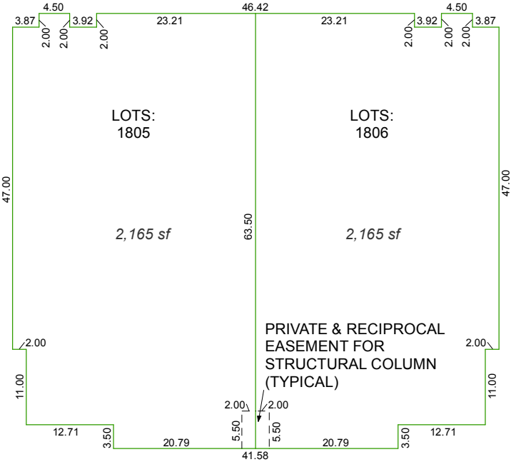
LOT DETAIL "D"
