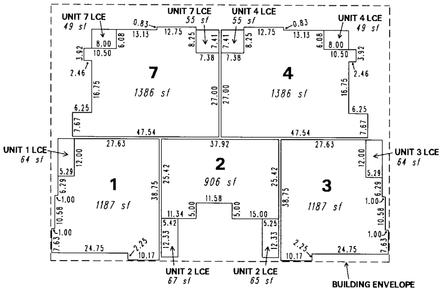
SECOND FLOOR
