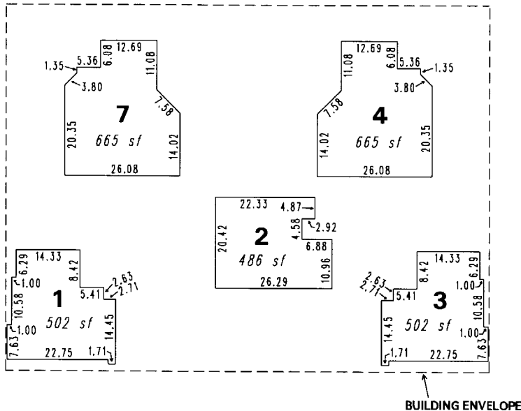
LOFT FLOOR
