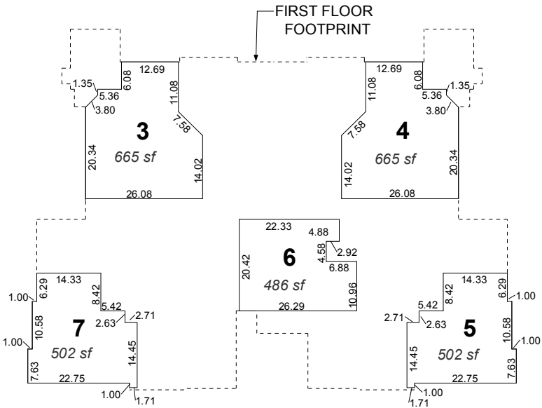
LOFT FLOOR PLAN
