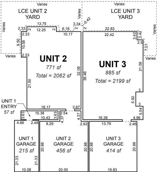
BUILDING TYPE C FIRST FLOOR
