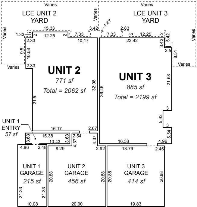
BUILDING TYPE A FIRST FLOOR
