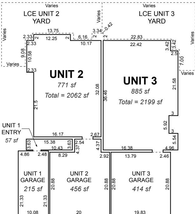
BUILDING TYPE B FIRST FLOOR
