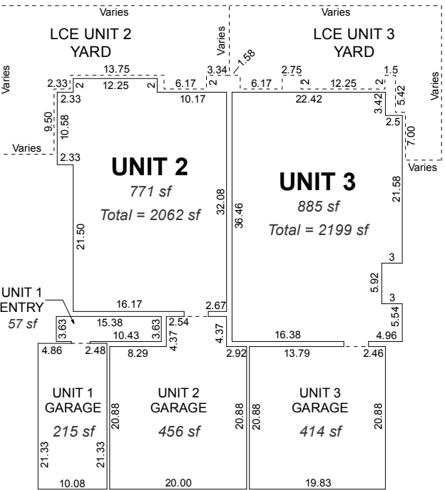
BUILDING TYPE D FIRST FLOOR
