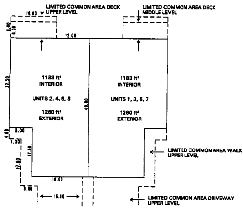
UNITS 1-8 MIDDLE / UPPER FLOOR PLAN SCALE: 1" = 20'
