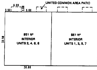
UNITS 1-8 LOWER FLOOR PLAN SCALE: 1" = 20'
