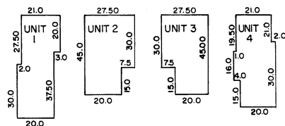
FIRST FLOOR
