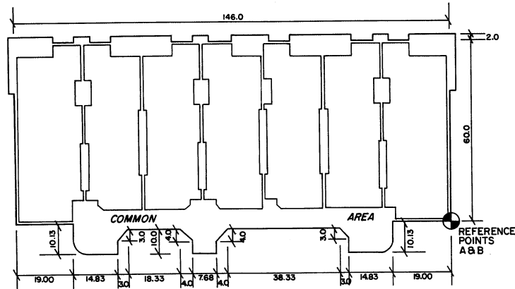
BUILDING PLAN
