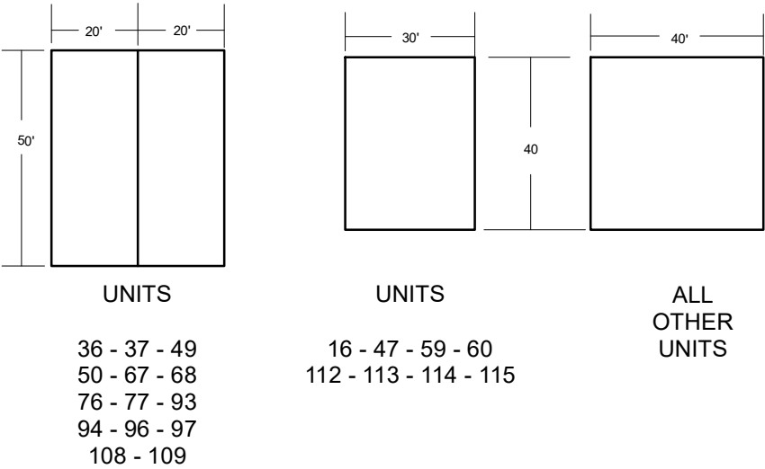
1" = 40' TYPICAL UNIT DIMENSIONS
