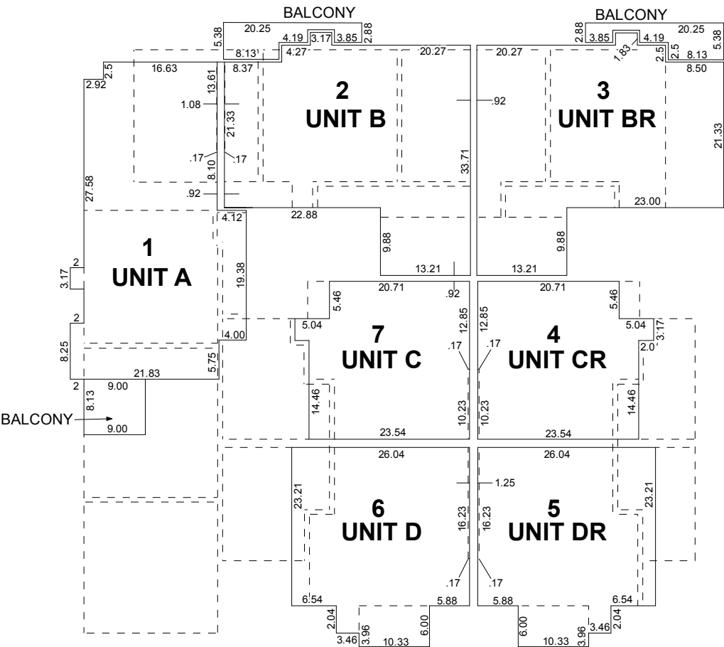
SECOND FLOOR
