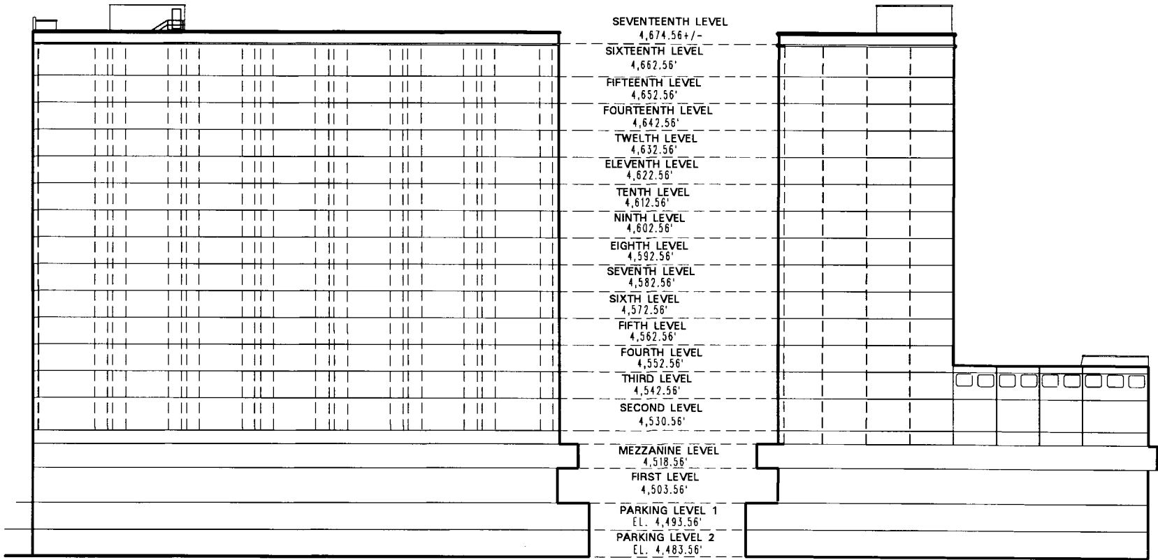
EAST ELEVATION
