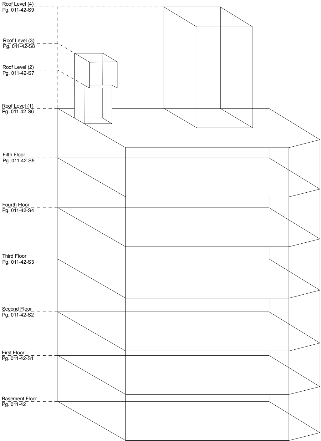
BUILDING DETAIL (not to scale)
