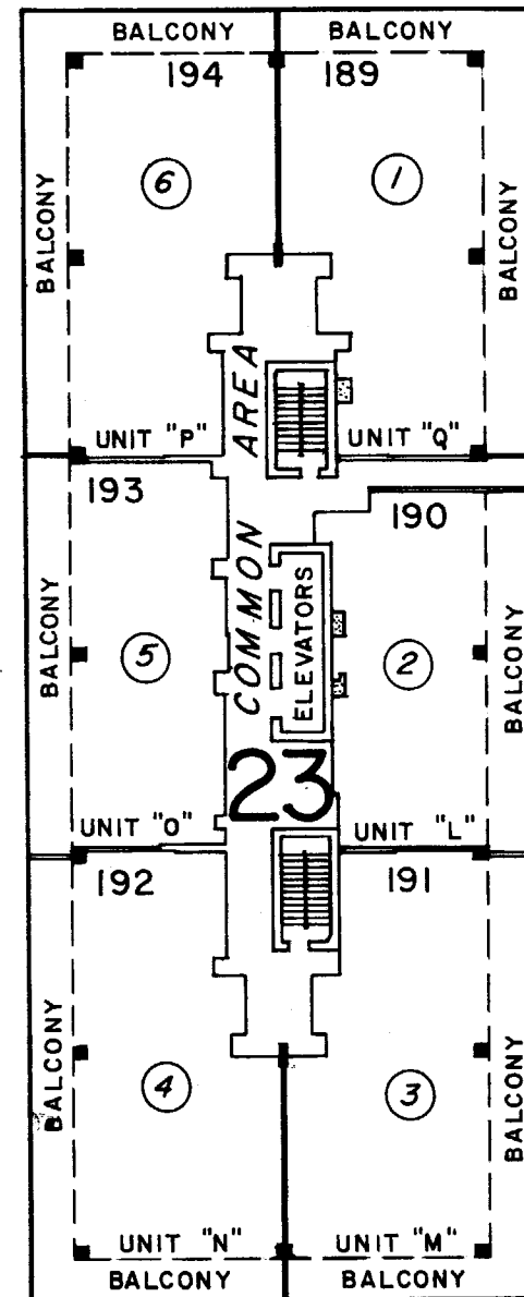
23 rd FLOOR
