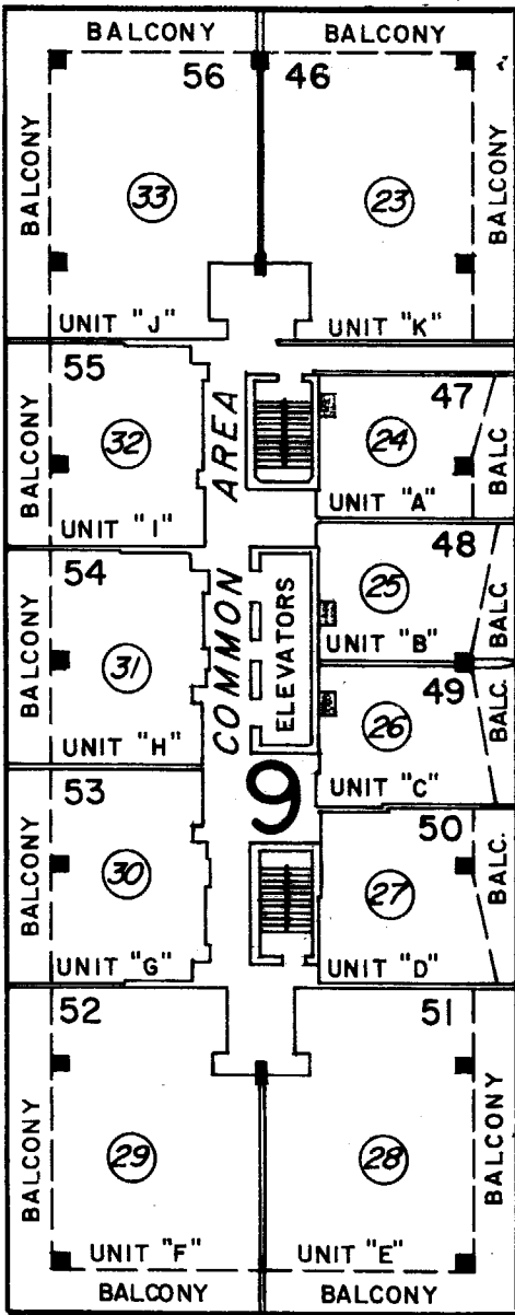
9 th FLOOR
