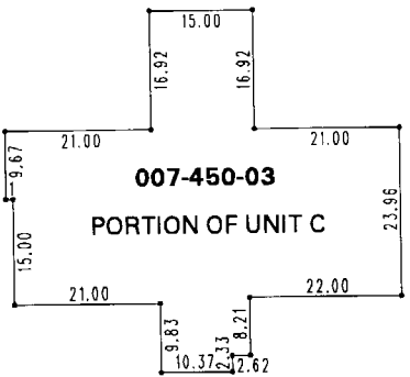
UPPER DETAIL
