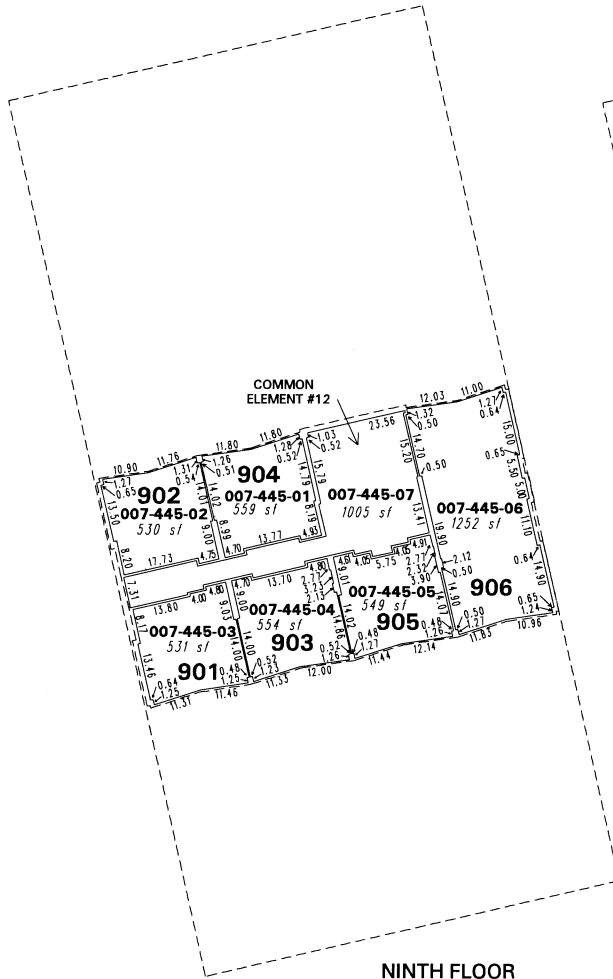
NINTH FLOOR
