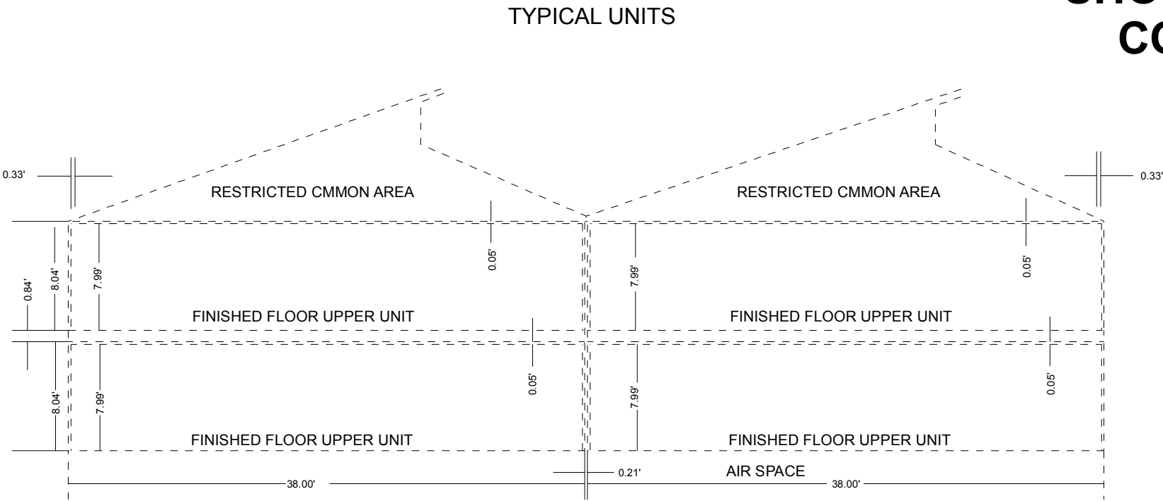
FRONT VIEW
