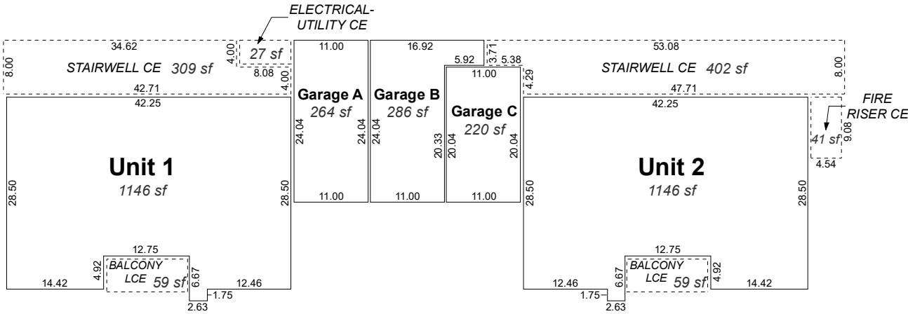
BUILDING TYPE 2A FLOOR ONE
