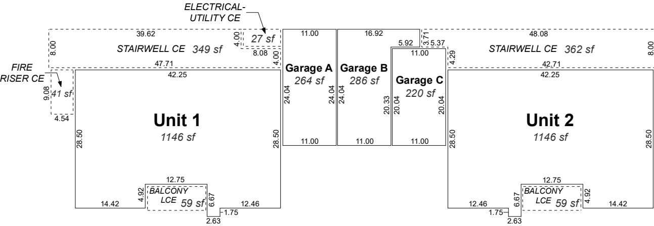
BUILDING TYPE 2 FLOOR ONE
