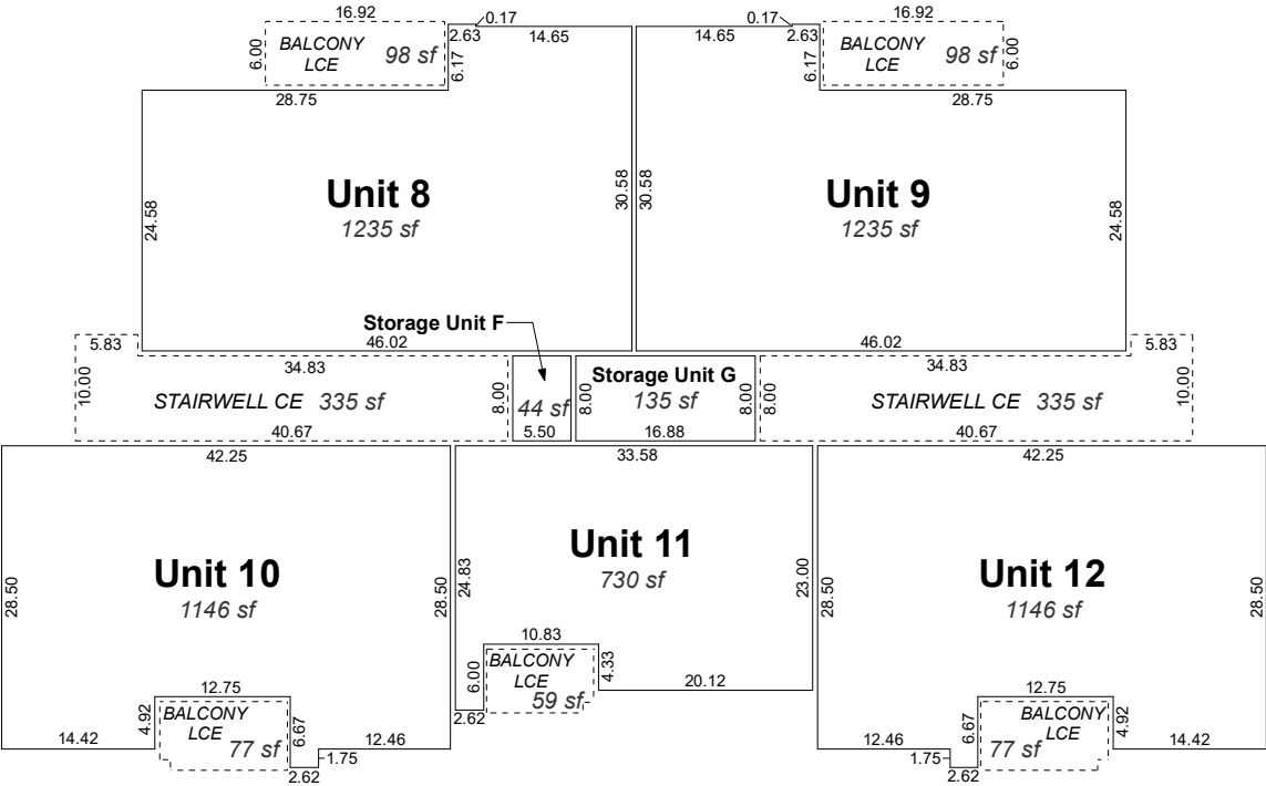
BUILDING TYPE 2 & 2A FLOOR THREE
