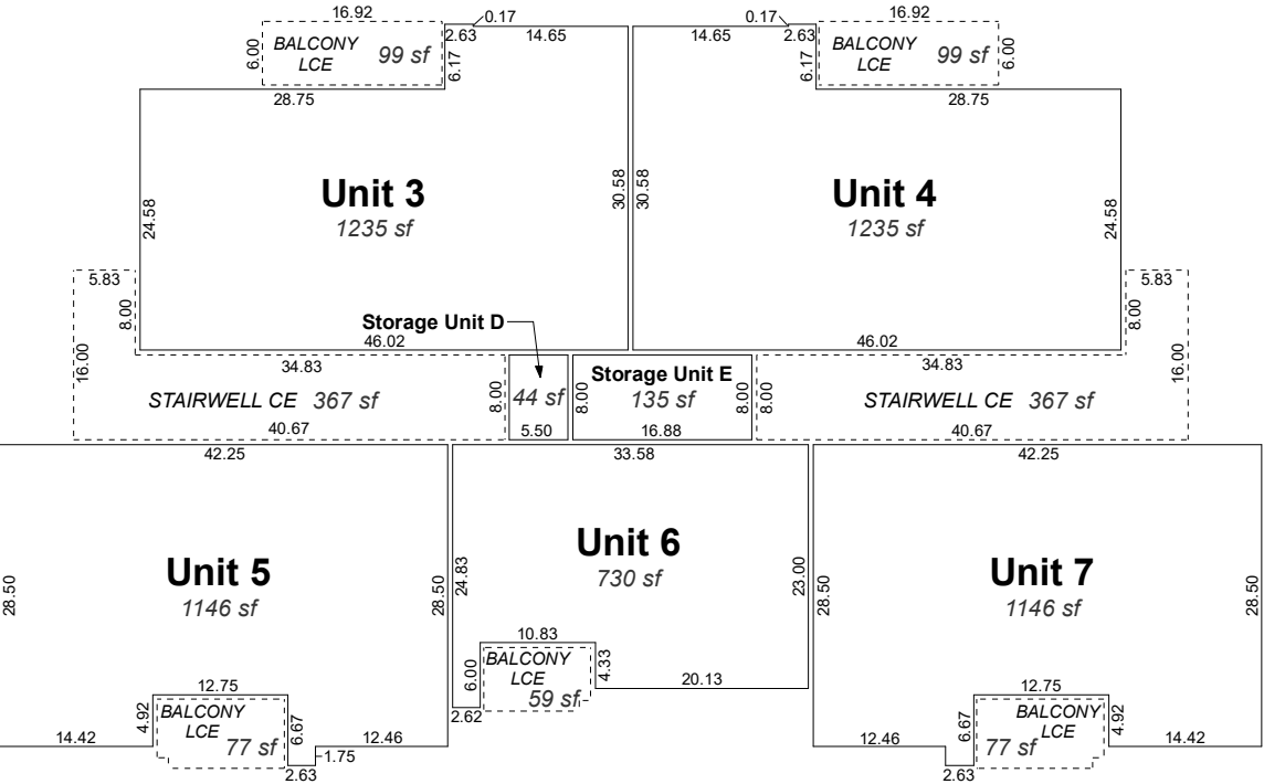
BUILDING TYPE 2 & 2A FLOOR TWO
