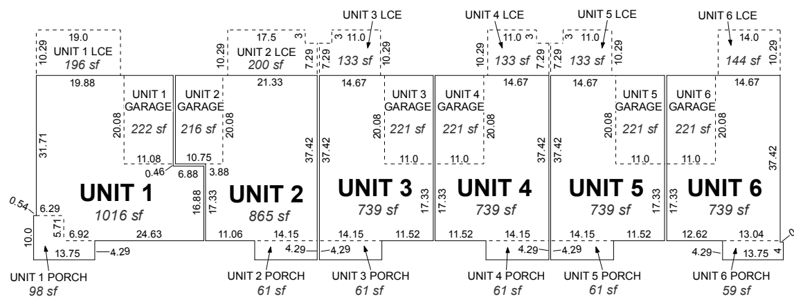
BUILDINGS 27, 28, 29, 42 & 46 ( 6-UNIT BUILDING )
