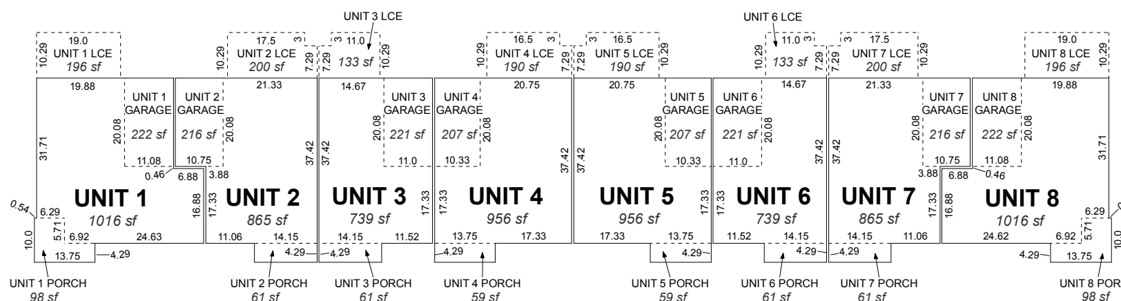
BUILDINGS 30, 31, 32, 33, 34, 35, 36, 37, 38, 39, 40, 41, 43, 44 & 45 ( 8-UNIT BUILDING )
