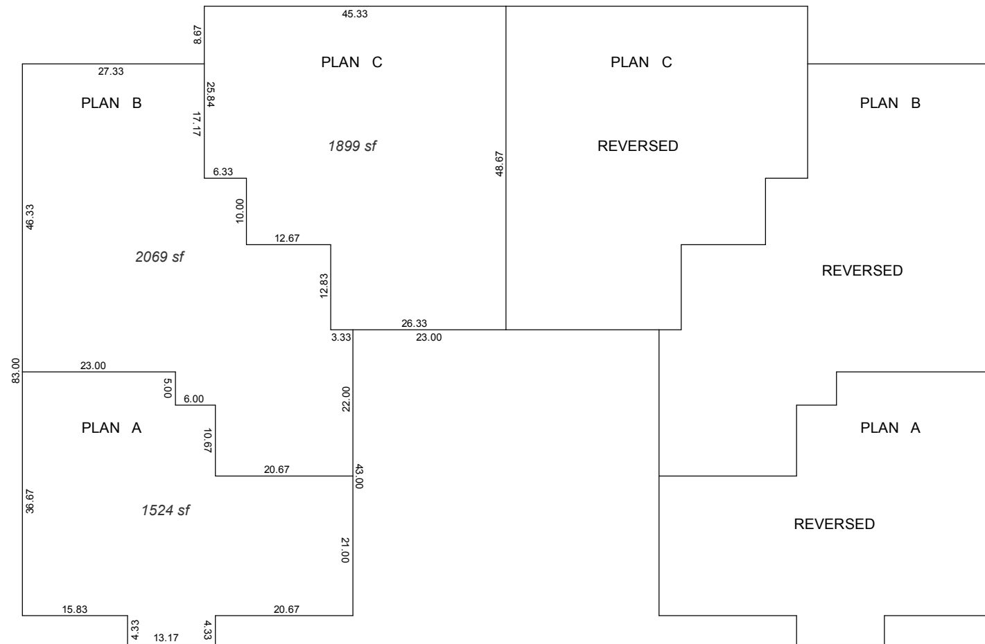
TYPICAL UNIT DIMENSIONS SCALE: 1" = 20'
