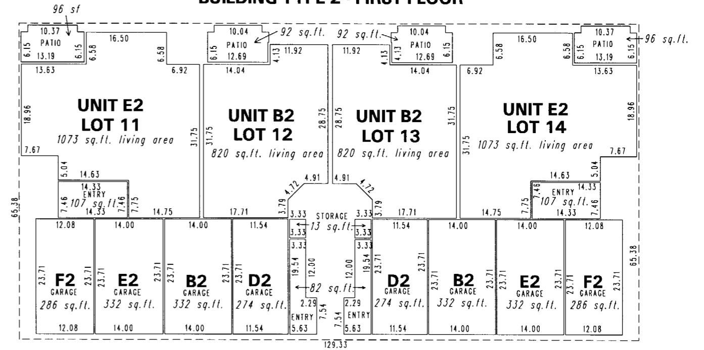
BUILDING TYPE 2 - FIRST FLOOR
