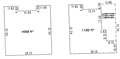
TYPICAL UNIT (EXCEPT UNIT 4) SCALE: 1" = 30'
