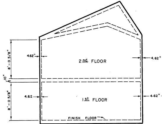
BUILDING TYPE "A"
