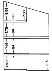
SECTION UNIT 1 (UNIT 2 IS OPPOSITE)
