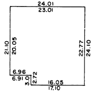
FIRST FLOOR UNITS 1 & 3 (UNITS 2 & 4 ARE OPPOSITE)
