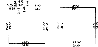
THIRD FLOOR UNIT 1 (UNIT 2 IS OPPOSITE)
