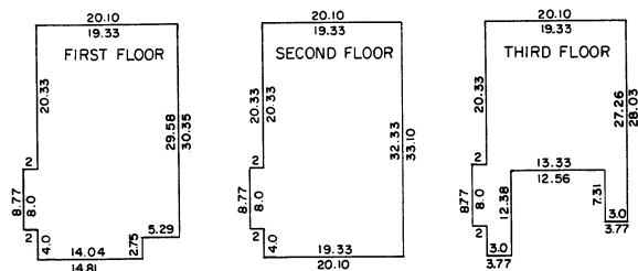
UNITS 1 & 4 (UNIT NO.1 IS OPPOSITE)
