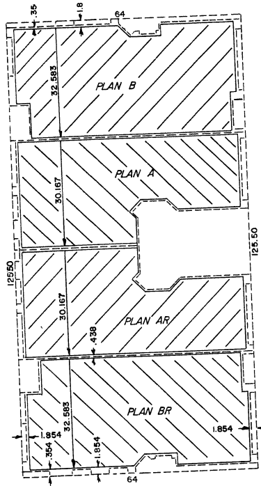
PLAN VIEW NTS
