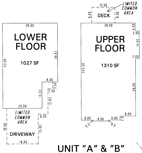
TYPICAL UNITS SCALE 1" = 20'
