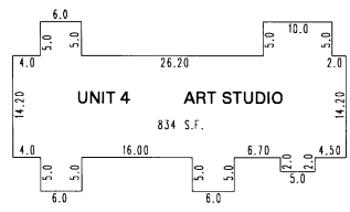
SECOND FLOOR PLAN - GARAGE
