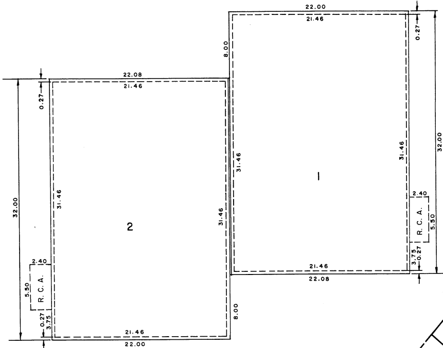
FLOOR PLANS SCALE: 1/8" = 1'-0" R.C.A. = RESTRICTED COMMON AREA
