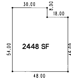
UNIT DIAGRAM FOR UNITS 1, 3 & 4
