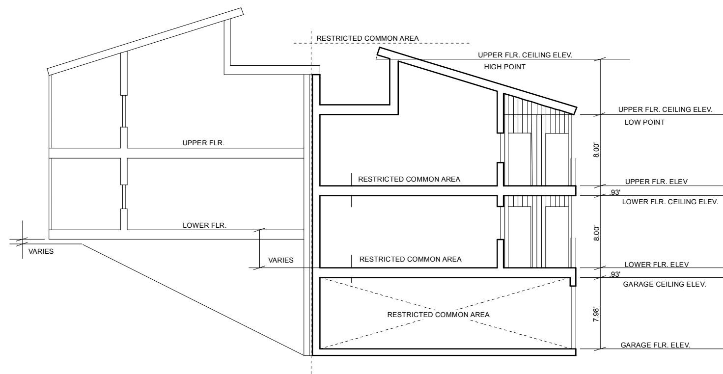
TYP. CROSS SECTION TWO AND THREE BEDROOM UNITS (NOT TO SCALE)
