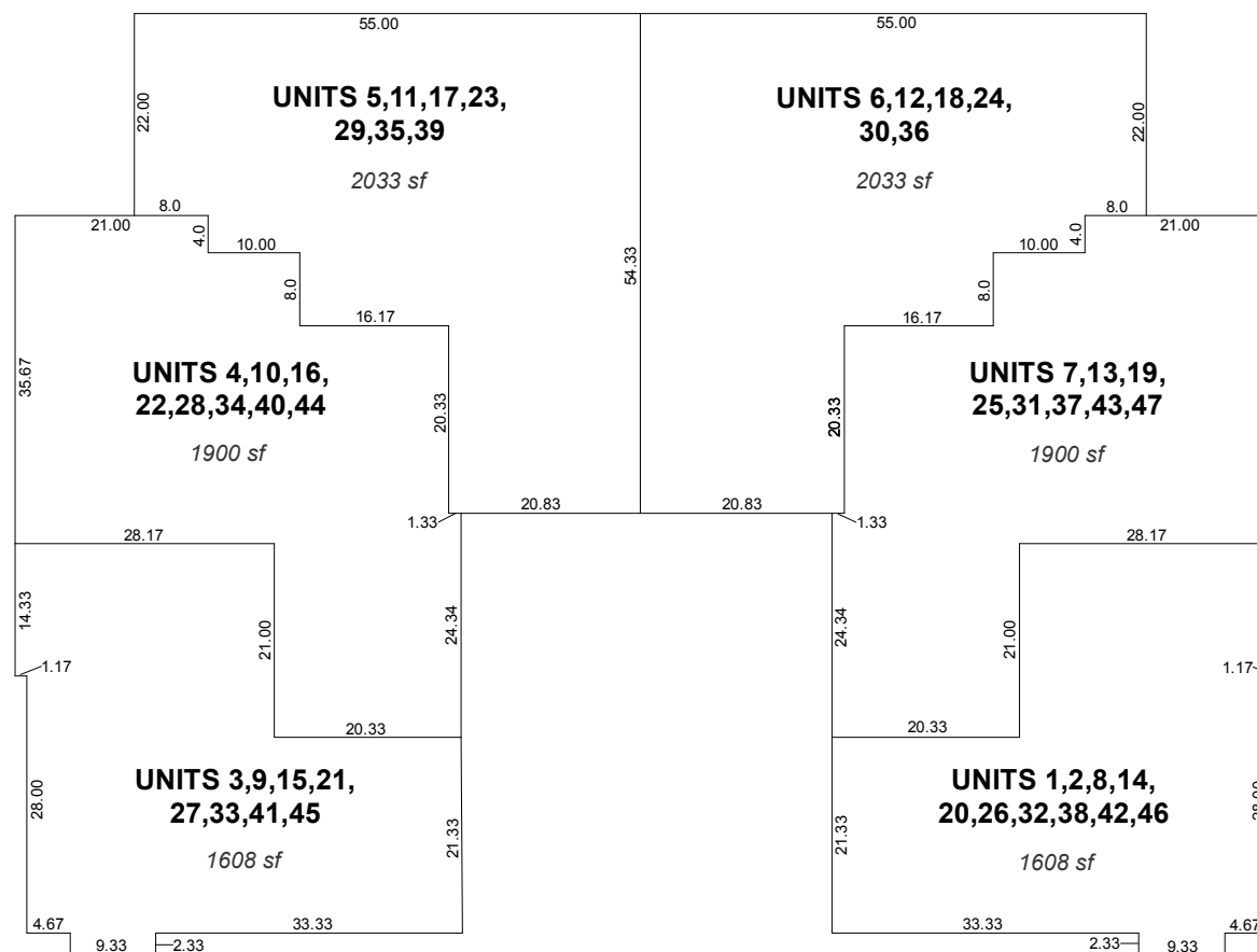
LOT DETAIL - NOT TO SCALE
