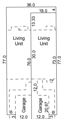
BLOCK D
