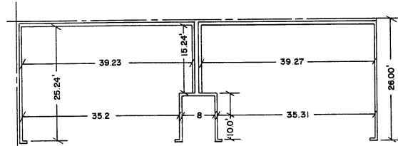
TYP. INTERIOR UNIT TYP. END UNIT TYP. AIR SPACE DIMENSIONS AT GARAGE (RESTRICT COMMON AREA)
