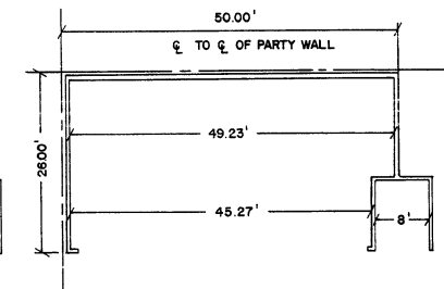
TYP. INTERIOR UNIT
