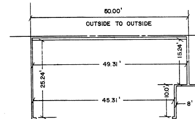
TYP. END UNIT DIMENSION FOR BUILDING 'I' ONLY
