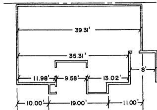
TYP. END UNIT AIR SPACE DIMENSIONS FOR BUILDING 'B' ONLY
