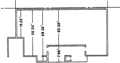
TYP. CROSS SECTIONAL DIMENSIONS FOR BUILDINGS G, H, I, J, K, L, M, N, O.
