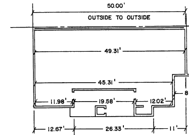
TYP. END UNIT DIMENSION FOR BUILDING 'I' ONLY
