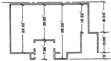
TYP. CROSS SECTIONAL AIR SPACE FOR BLDGS. G, H, I, J, K, L, M, N, O.
