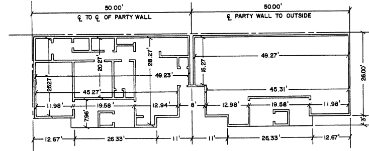
TYP. INTERIOR UNIT DIMENSION TYP. END UNIT DIMENSION FOR BUILDINGS A, C, E, F.
