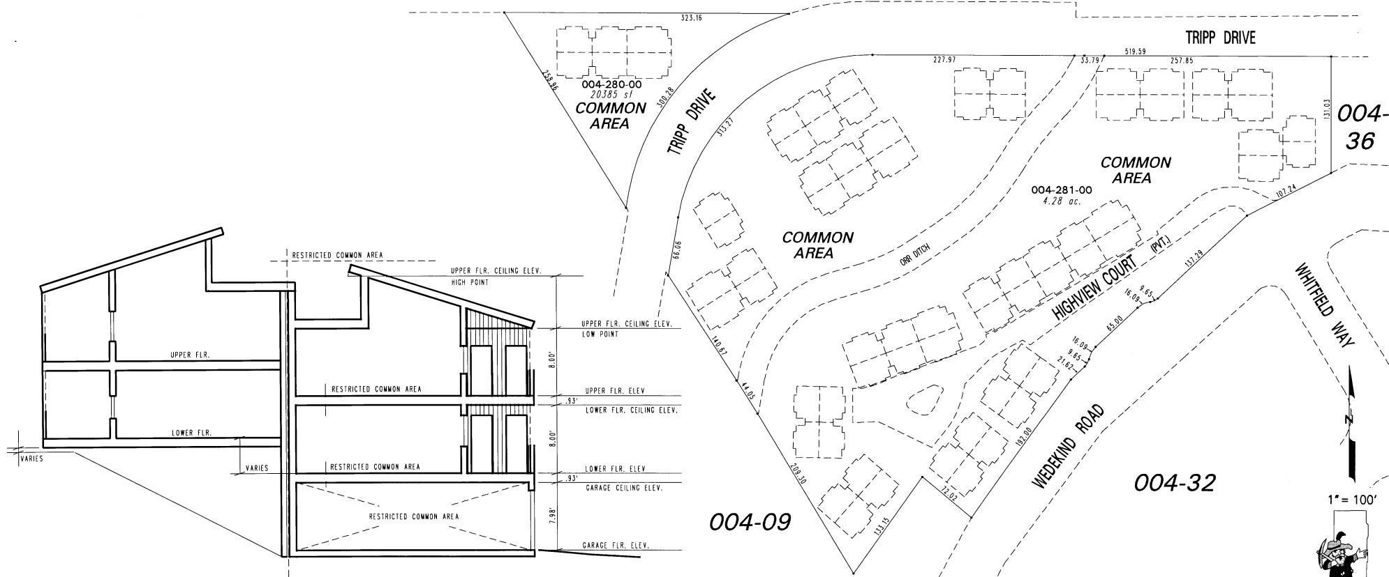
TYP. CROSS SECTION TWO AND THREE BEDROOM UNITS (NOT TO SCALE)
