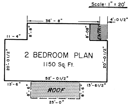
TYPICAL UNIT 1
